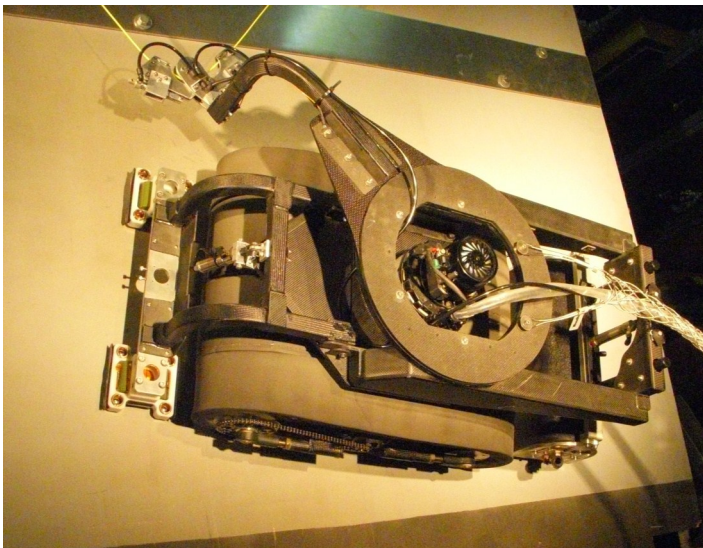
ICM Climber with Cleaning Brush and EMAT Tools
