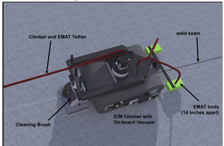
ICM Climber with Cleaning Brush and EMAT Tools
